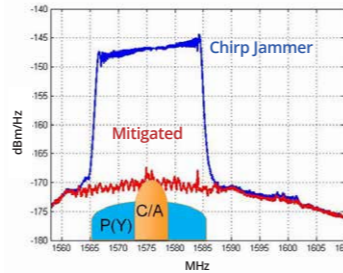
Figure 12 – GPS L1 signal contaminated with a chirp jammer signal: before (blue) and after (red) activation of WIMU (Wide-band Interference Mitigation Unit)
