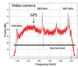
Figure 6 – L1-band Interference from a GoPro™ Hero 2 video camera picked up by GPS antenna
