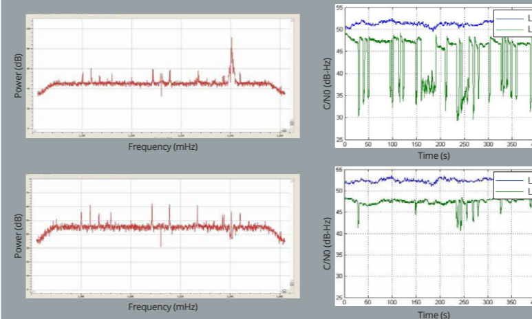
Figure 10 Observed L1 and L2 signal power before enabling AIM+ showing significant impairment of L2 C/N0
