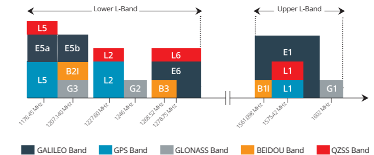
Figure 2 – RF spectrum for GNSS
