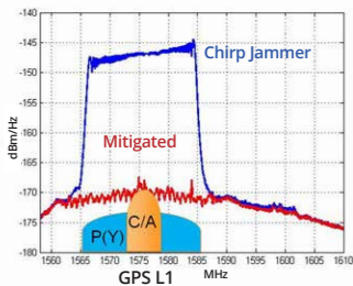
Figure 4 – GPS L1 signal contaminated with a chirp jammer signal: before (blue) and after (red) activation of WIMU (Wide-band Interference Mitigation Unit)
